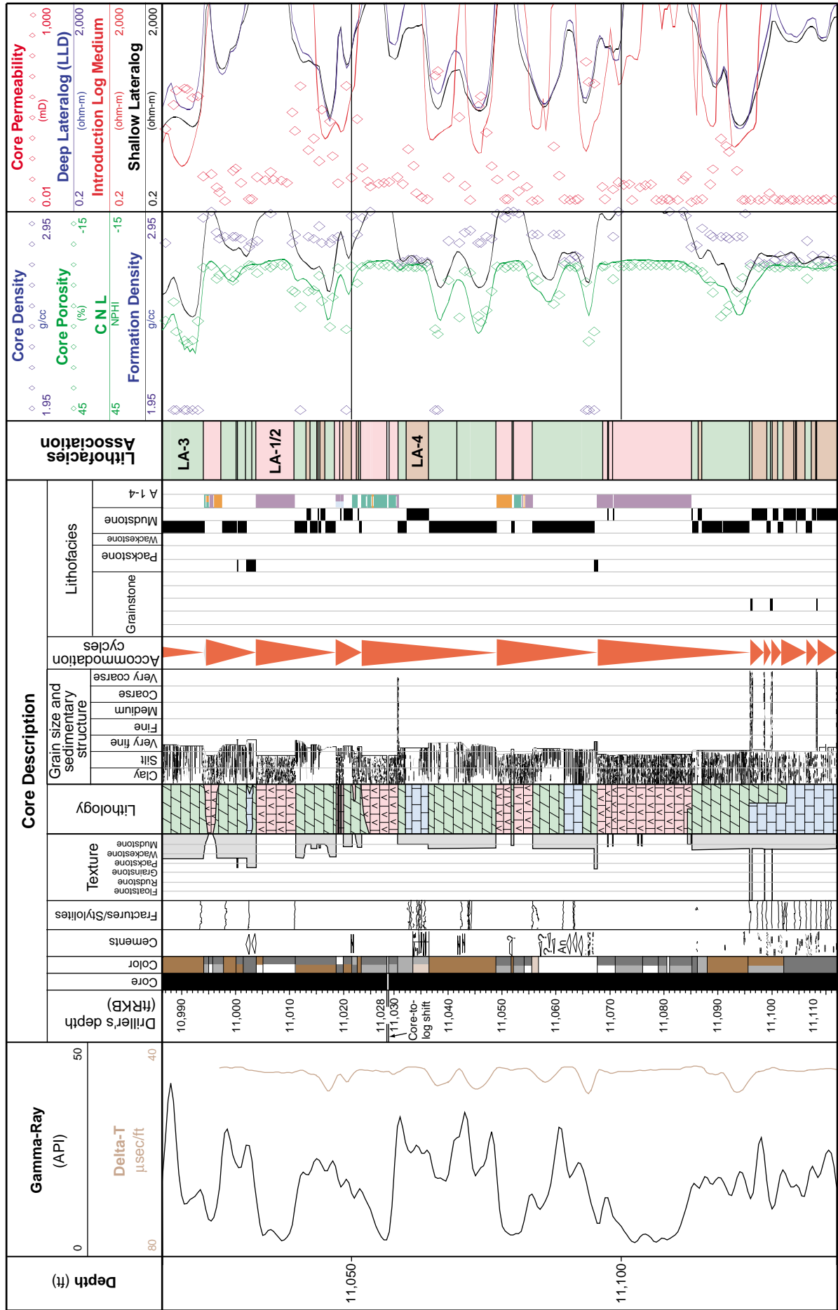
Figure 7a: Typical core and log expressions of the Arab-ABC shallowing-upward cycles for the various lithofacies associations.
