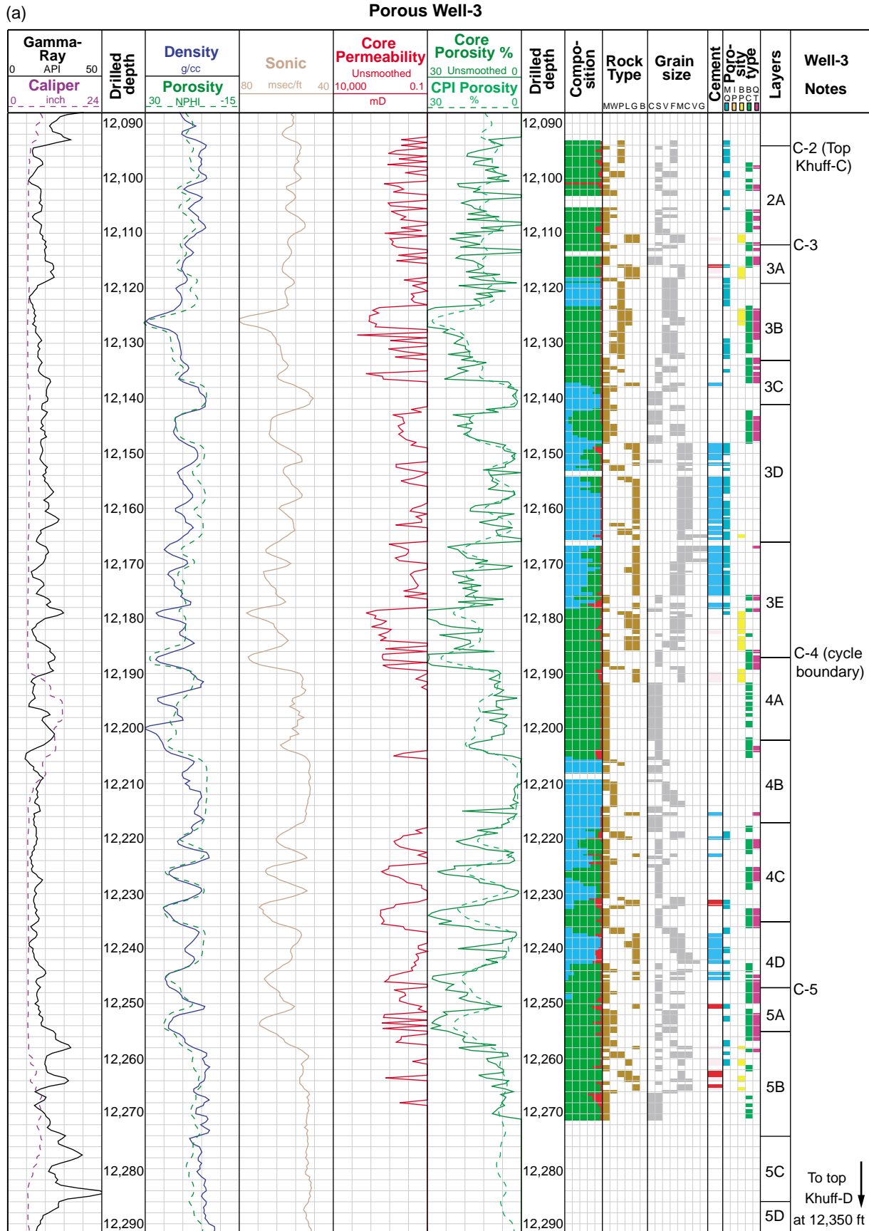
Figure 6: Core logs from Khuff-C: (a) porous well-3 and (b) tight well-B. In (a) porous Khuff-C consists of grainstone and some dolomite with up to 30 percent core porosity; in (b) tight Khuff-C has a dolomite matrix with pores filled with anhydrite cement.
